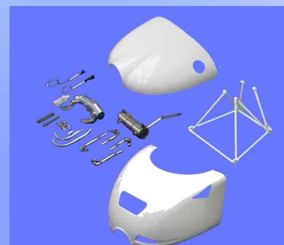
Rotax 912 installation kit
