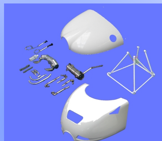
Rotax 912 installation kit
